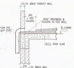
SECTION 3-3
