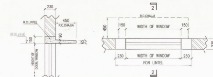
SECTION 2-2
