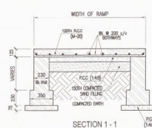
SECTION 1-1
