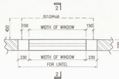
TYP. DET. OF LINTEL & CHAJJA
