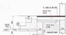
DET. OF STEPS FOR DOORS
