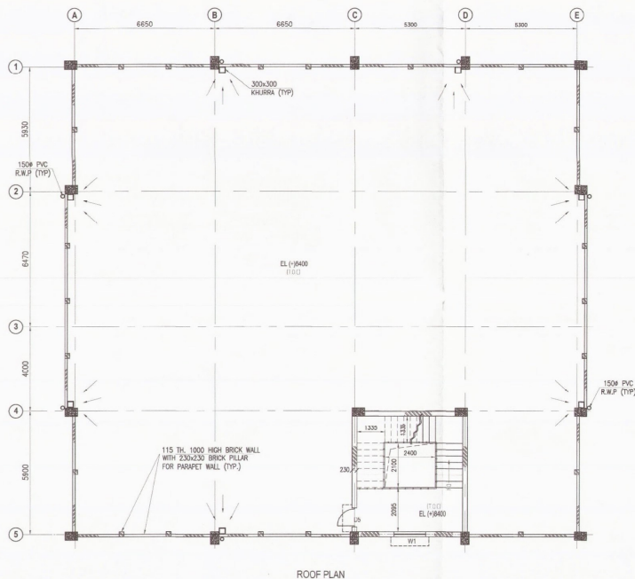
ROOF PLAN
